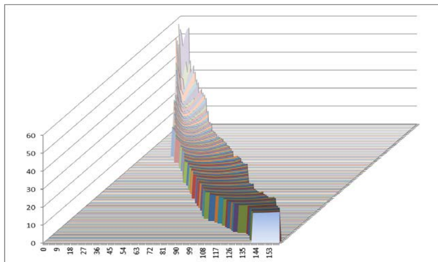
Figure 8: The Number of Remaining Defecton Averaged Per Nucleon in the Primary Nucleosynthesis of a Cloud of Isotopes from Relic Neutrons According to the Gamow Scheme (Rook - Rearview)
