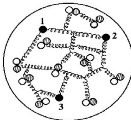
Figure 3: Quark-Gluon Model of Nucleons
