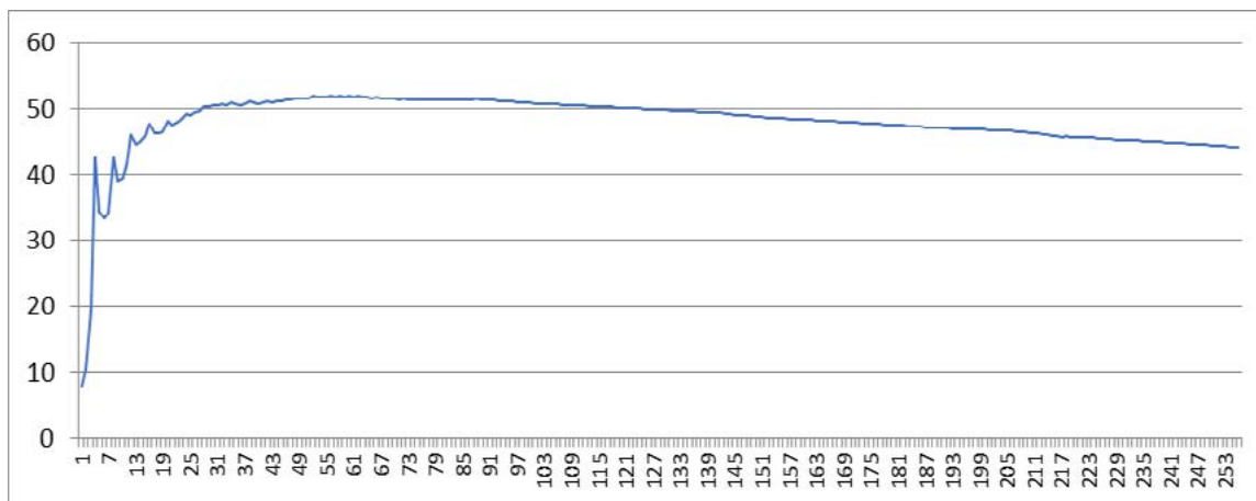
Figure 6: Average Number of Destroyed Defecton Per Nucleon
