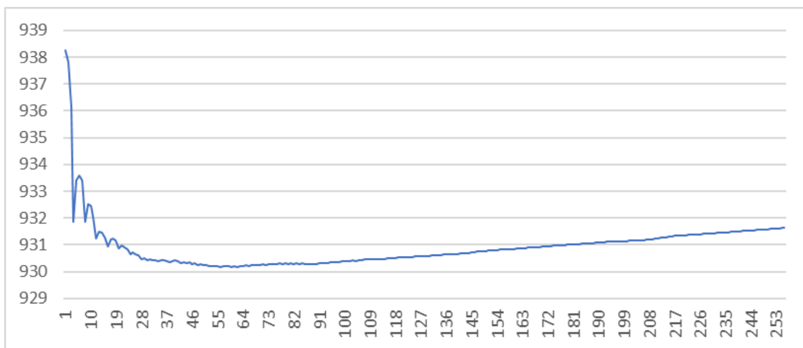
Figure 1: Average Mass of One Nucleon from the Number of Nucleons in the Isotope Nucleus (for Isotopes of the Valley of Stability)
