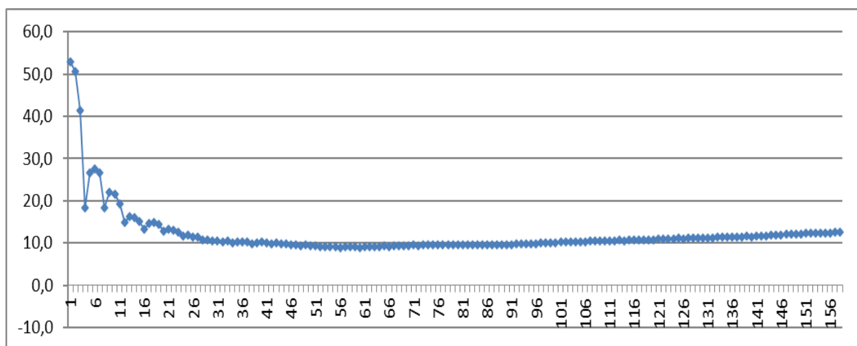
Figure 10: The Minimum Value of the Number of Defecton Remaining in the Isotope, Averaged Per one Nucleon, for Each Row of Isotopes (Stable Isotopes of a Chemical Element)
