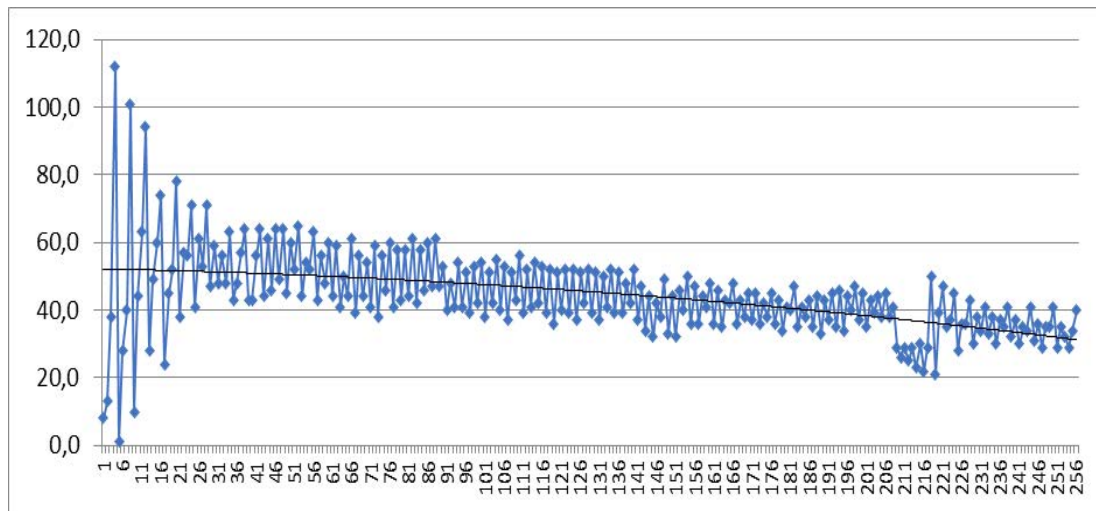
Figure 5: The Number of Destroyed Defecton at Each Step of the Primary Nucleosynthesis of Stable Isotopes with a Polynomial Trend Line (Main Stream)
