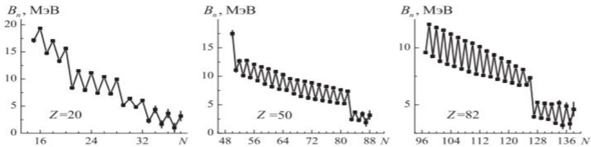
Figure 4: Dependence of the Neutron Separation Energy B_n on the Number of Neutrons N in the Isotopes Ca, Sn, and Pb
