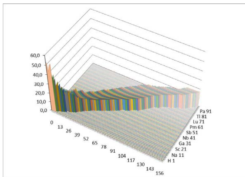
Figure 9: The Number of Remaining Defecton Averaged Per Nucleon in the Primary Nucleosynthesis of a Cloud of Isotopes from Relic Neutrons According to the Gamow Scheme (Rook-Rearview)
