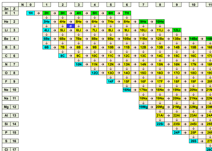
Figure 7: The Process of Primary Nucleosynthesis of an Isotope Cloud According to the Gamow Scheme
