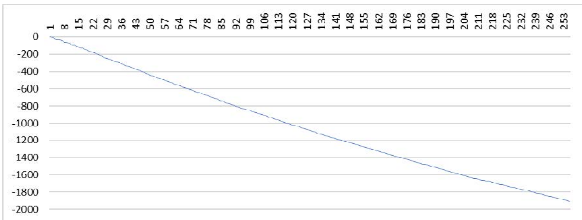
Figure 2: The Total Defect in the Mass of Nuclei of Isotopes on the Number of Nucleons in Nuclei (MeV)
